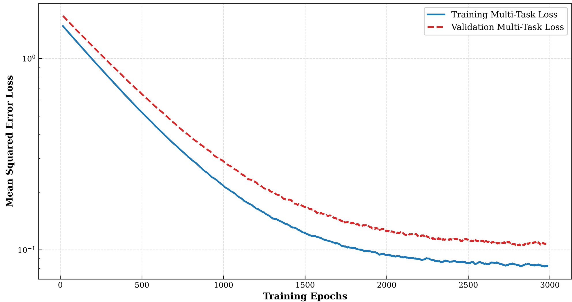
Multi-Task CGCNN Convergence Dynamics over 3,000 Epochs
